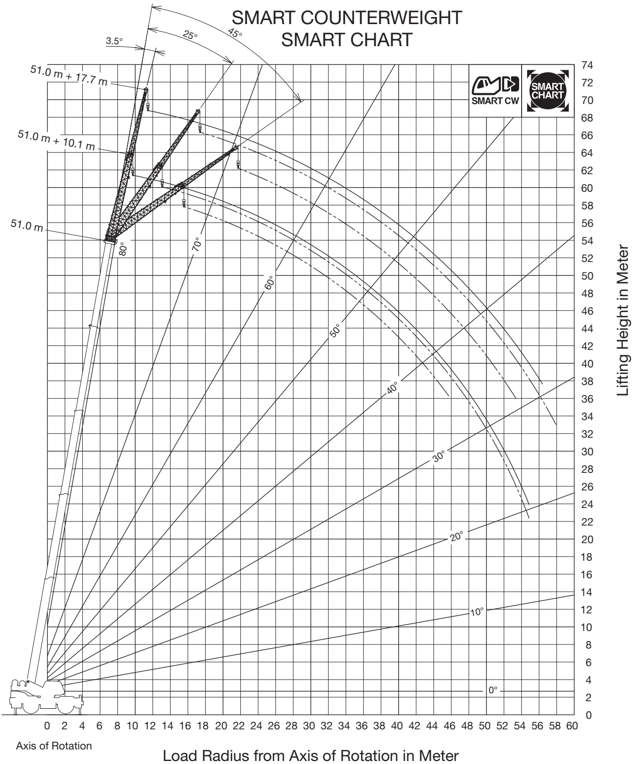
JIB
